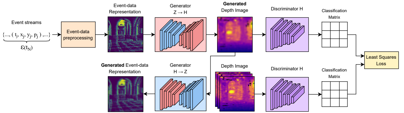
Fig. 3. Suggested CycleGAN architecture for event-based monocular depth estimation baseline. Event streams are preprocessed into dense representations, which are then translated into depth images and back through paired generators ( H \rightarrow Z , Z \rightarrow H ). Discriminators enforce realism in each domain using a least-squares loss, while cycle consistency enables reconstruction across event and depth domains.
